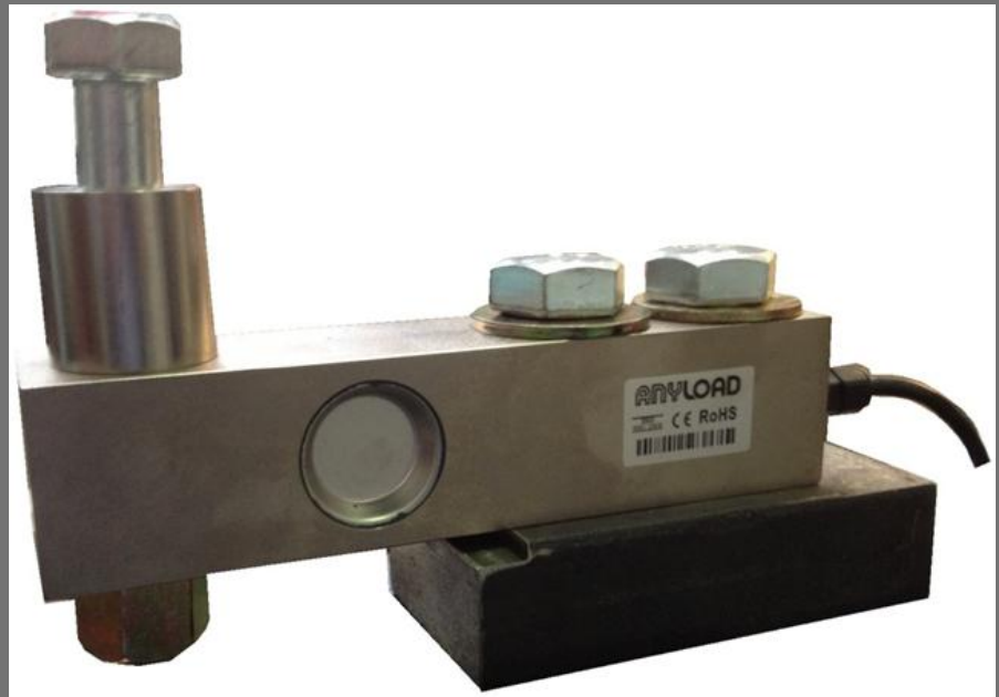
Picture of ASCI Weigh Mount with 5t 563YH Load Cell Weighing Mount designed and Manufactured in Australia by Associated Scale Service
