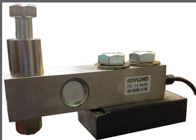
Shows an ASCI Weigh Mount with 5t 563YH Load Cell
